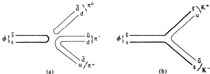
FIG. 4.10. \phi decays: (a) disallowed; (b) allowed by the Zweig rule.
