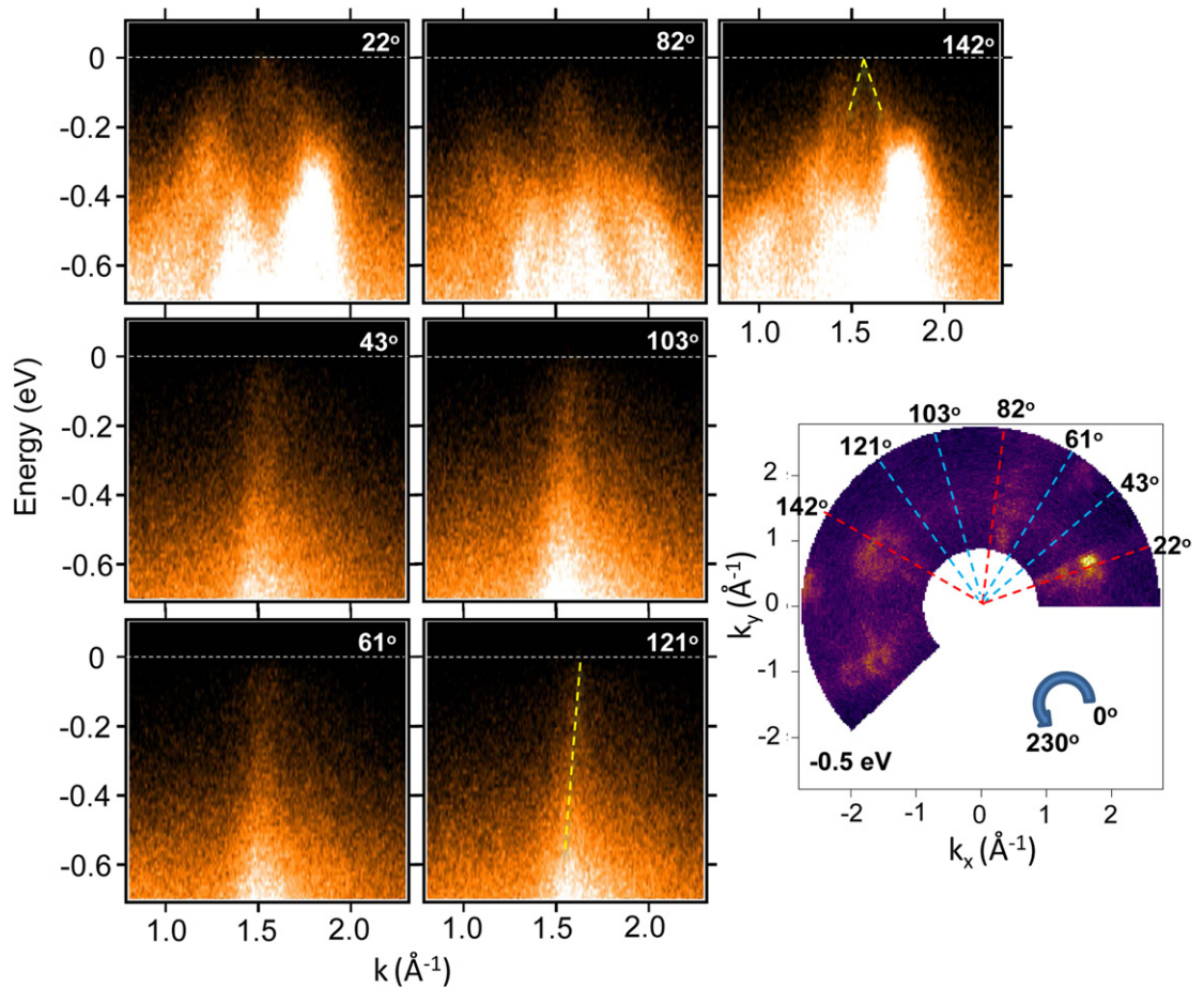
Figure 4. ARPES spectral cuts at different azimuthal angles showing the coexistence of topological surface Dirac fermions of \text{Sb}_2\text{Te}_3 and Dirac \pi bands of graphene. The dashed lines serve as a guide to the eye, showing the dispersion of TI Dirac surface states and graphene \pi bands.
