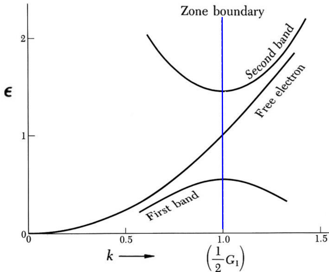
Figure 9 Solutions of (50) in the periodic zone scheme, in the region near a boundary of the first Brillouin zone.
