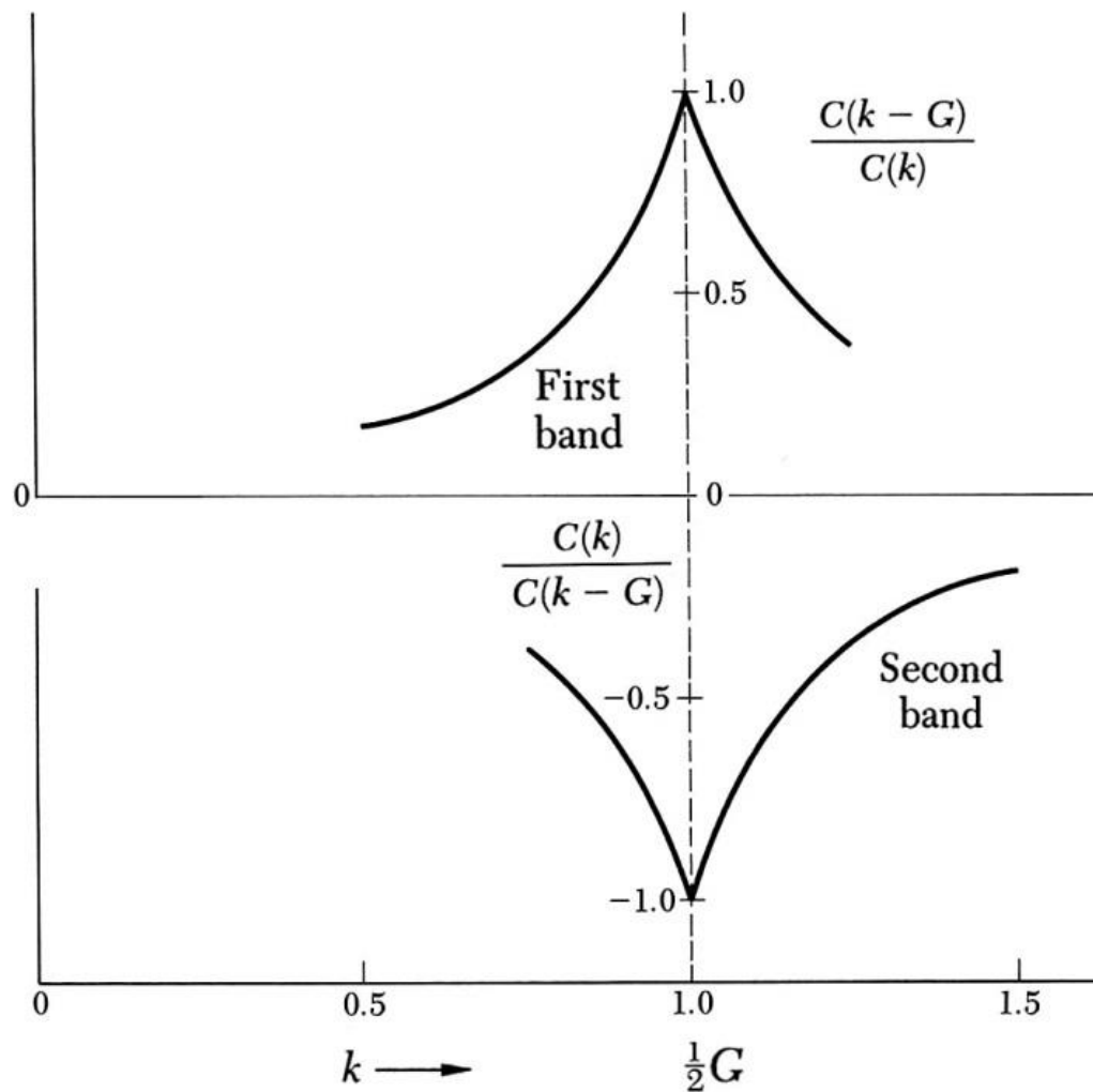
Figure 10 Ratio of the coefficients in \psi(x) = C(k) \exp(ikx) + C(k-G) \exp[i(k-G)x] as calculated near the boundary of the first Brillouin zone. One component dominates as we move away from the boundary.
