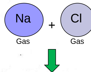
Figure 8 The energy per molecule unit of a crystal of sodium chloride is (7.9 - 5.1 + 3.6) = 6.4 eV lower than the energy of separated neutral atoms. The lattice energy with respect to separated ions is 7.9 eV per molecule unit. All values on the figure are experimental. Values of the ionization energy are given in Table 5, and values of the electron affinity are given in Table 6.
