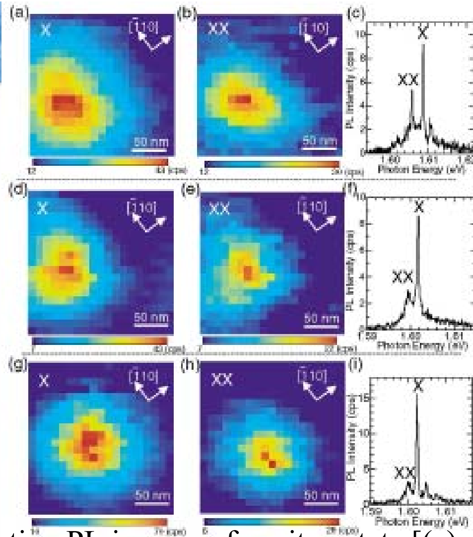
(a) –(i) Series of high-resolution PL images of exciton state [(a), (d), and (g)], biexciton state [(b), (e), and (h)], and corresponding PL spectra [(c), (f), and (i)] for three different QDs. Scanning area is 210 \times 210 \text{ nm}^2 . Crystal axes along 110 and 1\bar{1}0 directions are indicated. PL image sizes of biexciton are always smaller than those of exciton.
