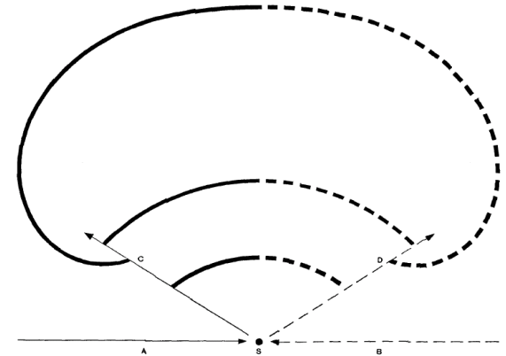
Figure 1 Schematic representation of current flow disturbed by the scatterer S. Electrons in excess numbers are incident along A, then are scattered to C, then scattered by the background. The number of electrons incident along B is less than the equilibrium number. The deficit is scattered to D, then scattered by the background. The excess and deficit diffuse together and recombine along the arcs.
