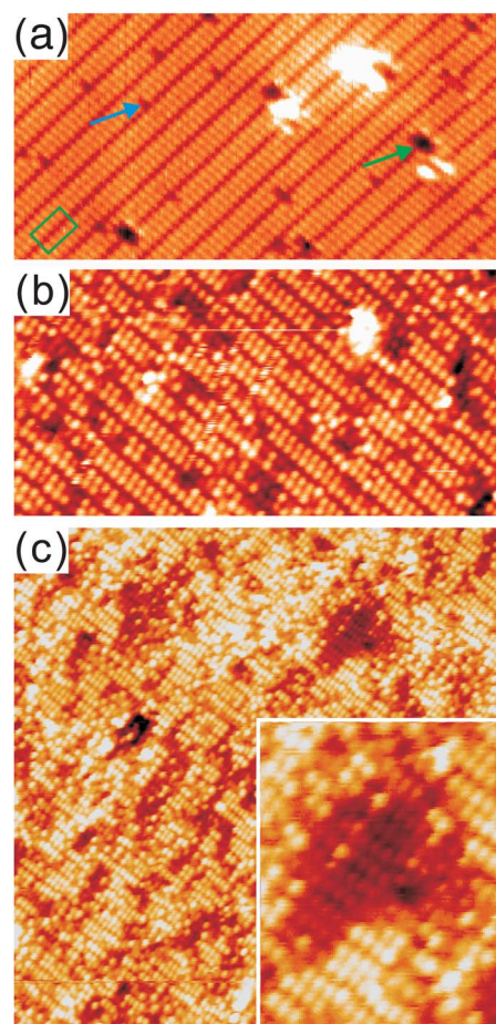
FIG. 3. (Color online) STM images of the Cl/Si(100)-2 × 1 surface after (a) 0, (b) 36, and (c) 90 L apparent dosages of H atoms. The sample bias used was +2 V. In (a) the green rectangle box, running from the upper right to the lower left, encloses a row of five Cl–Si–Si–Cl (monochloride) species. A surface Cl atom appears as a bright protrusion and forms a narrow ellipse with another in the neighboring monochloride row in the image. Notably each of two nearest Cl adatoms in the empty state images are not from a single Cl–Si–Si–Cl species, but are a part of two adjacent Cl–Si–Si–Cl species. The green and blue arrows point to a missing dimer defect site and a H-termination site, respectively. The inset in (c) shows a 2 × 1 area of nearly complete H termination after Cl extraction. The size of a 1 × 1 unit cell in the image is 3.84 \times 3.84 \text{ \AA}^2 .
